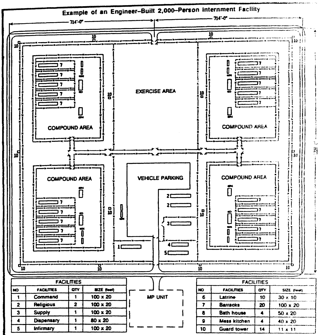
Figure 3-4. EPW/CI Enclosure.
